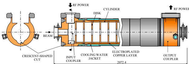
Figure 1: Schematic of the accelerating structure.
